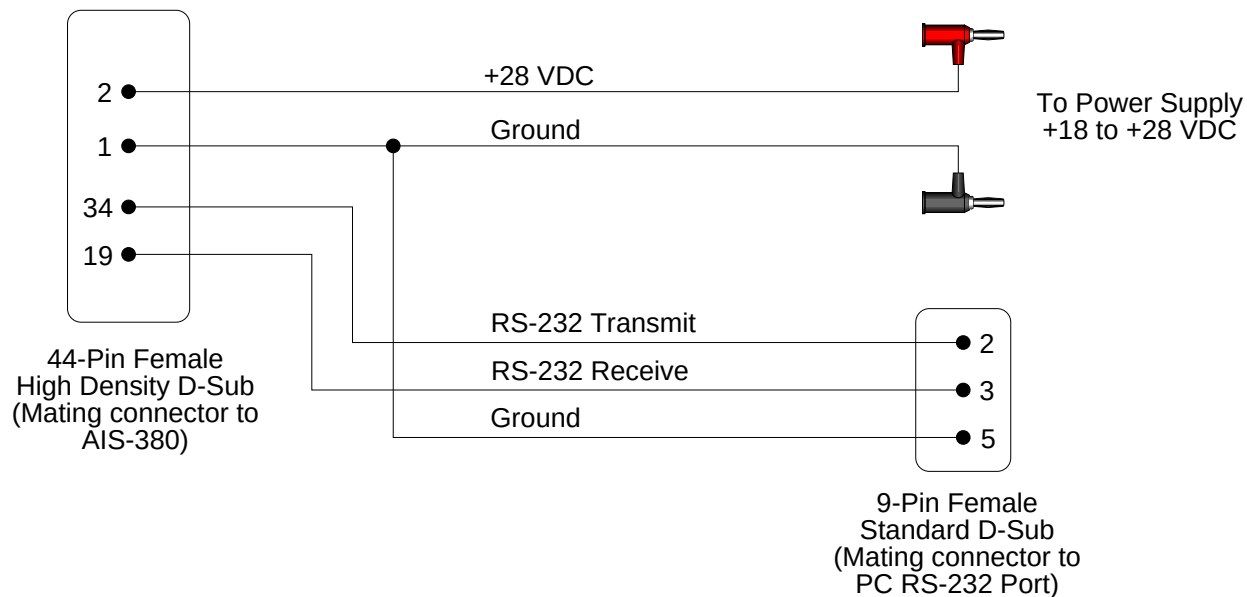
Figure 4 : Field Configuration Cable
