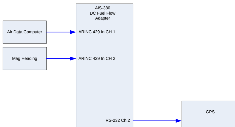
Figure 2 : Air Data Computer/Heading ARINC 429 to RS-232
